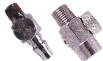
N52-20PMA / N-502 1/4" Air Flow Control Valve
